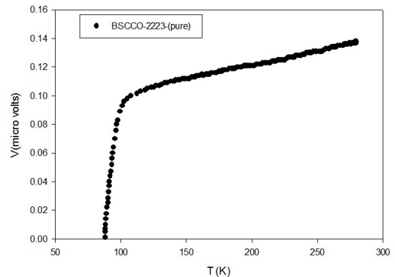
Fig 5. Electrical measurement vs. T for BSCCO-2223 (pure).
