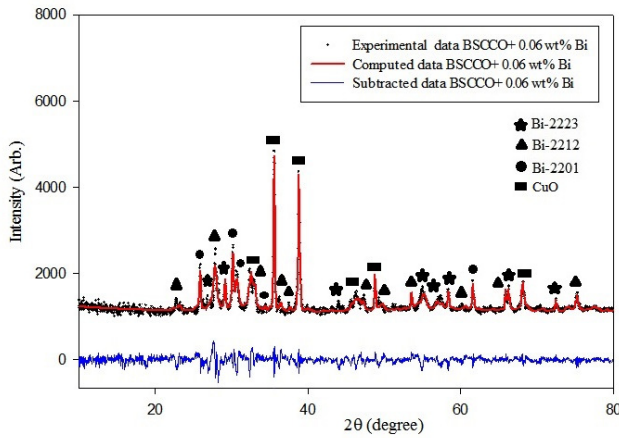
Fig 3. XRD of BSCCO-2223+ 0.06wt% Bi sample.
