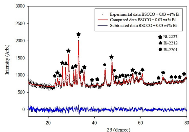
Fig 2. XRD of BSCCO-2223+ 0.03wt% Bi sample.
