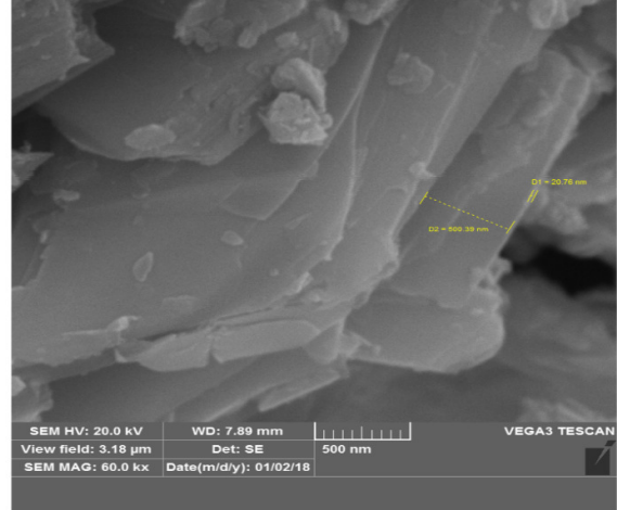
Fig 8. SEM image of synthesized BSCCO+0.03wt% Bi.
