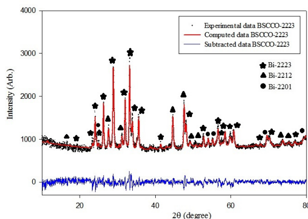
Fig 1. XRD of BSCCO-2223 (pure) sample.
