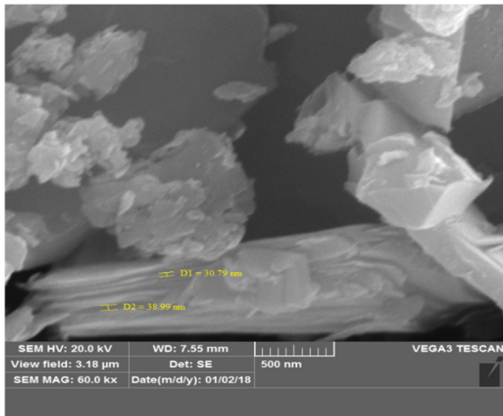
Fig 7. SEM image of synthesized BSCCO-2223 (pure).
