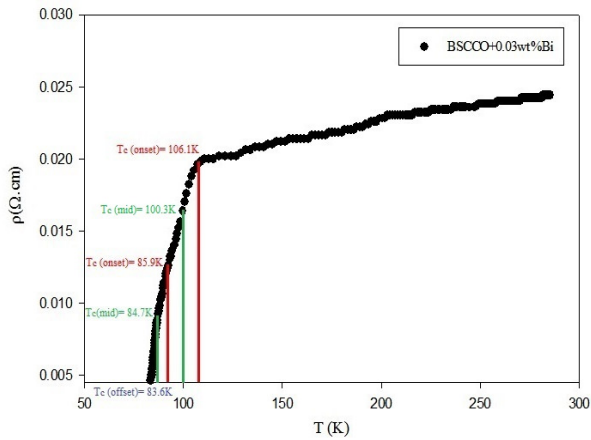
Fig 6. Electrical measurement \rho(T) for BSCCO+0.03wt% Bi.
