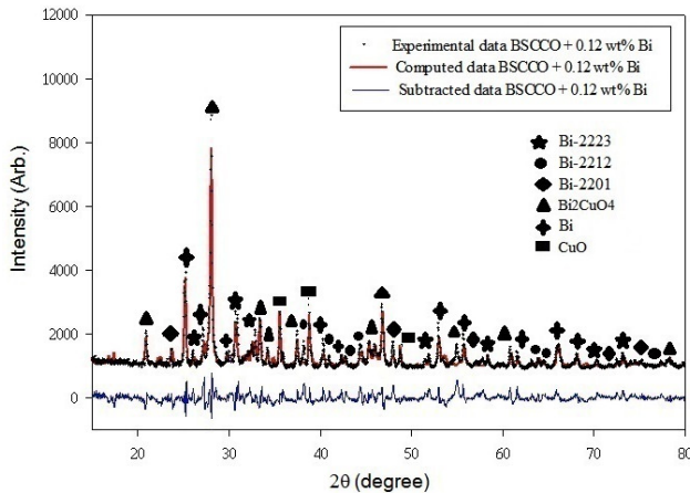
Fig 4. XRD of BSCCO-2223+ 0.12wt% Bi sample.
